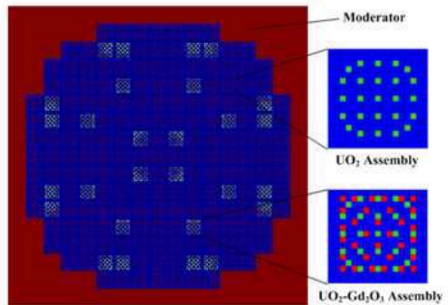
Fig. 1. X-Y View of the active core model with details assembly described on the side.
