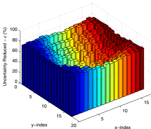
Fig. 3. FW-CADIS vs. GP.
